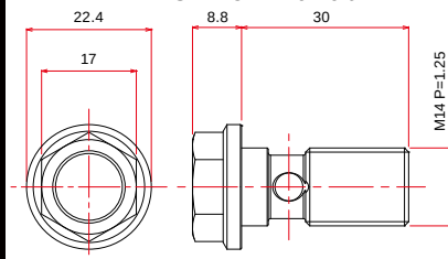
KAWASAKI Oil Line Bolt
