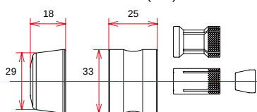
Universal L dimension (mm)
