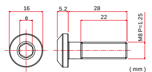
PAN HEAD Dimensions ZT11-1828
