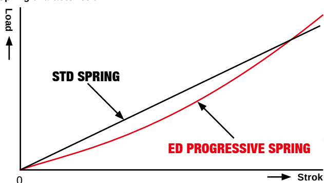
Spring characteristic
