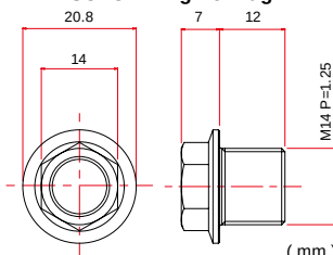
SUZUKI Engine Plug
