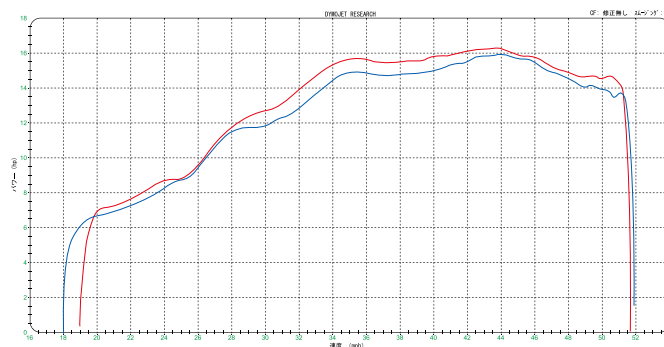
KLX230 Power Graph (hp)
