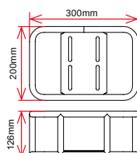
ALUMINUM FRONT CARRIER Dimension
